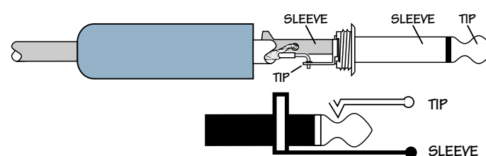
Figure C: TS Plug
