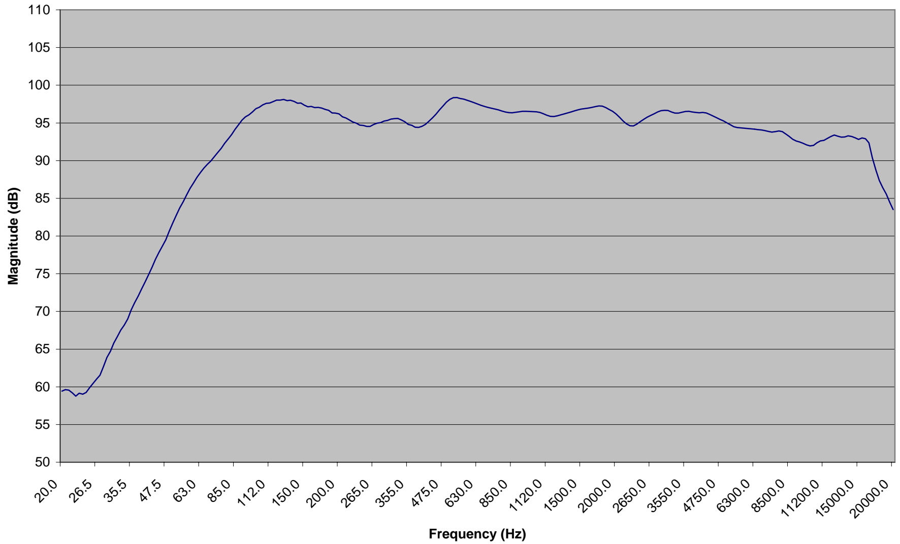
Axial Response (2.83V/1m)
