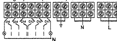
Single phase power input
