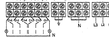
Three phase power input
