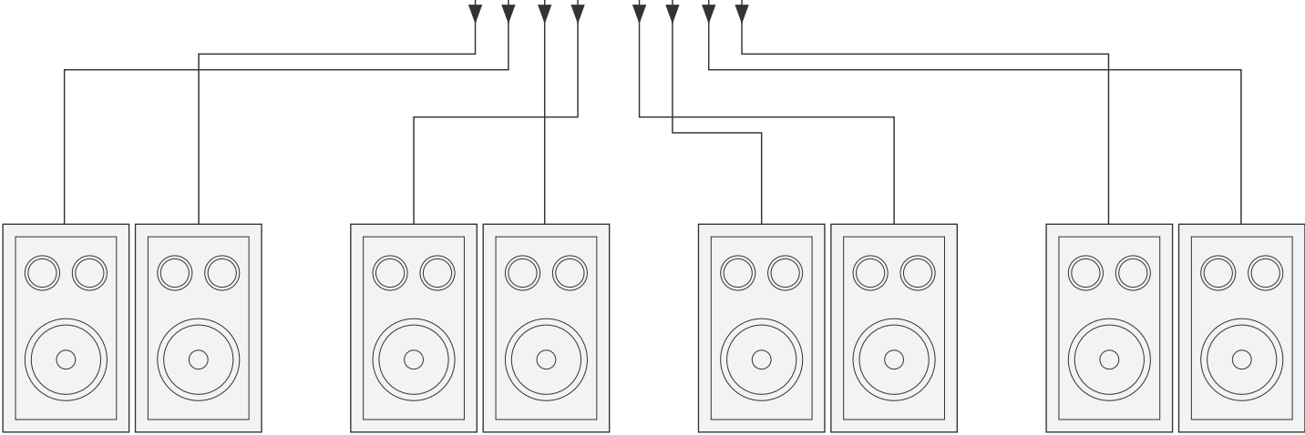
Stereo Speakers 4
