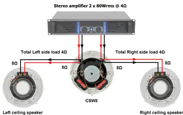
WIRING CSW8 AS PART OF A 2.1 STEREO SYSTEM
