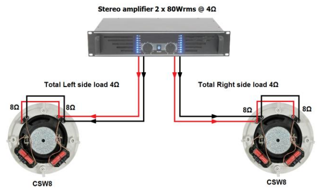
WIRING 2 X CSW8 AS 4Ω SUBWOOFERS
