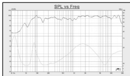
PHOBOS-15PSD SPL / IMPEDANCE VS FREQ.
