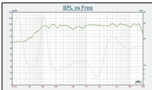
PHOBOS-12PSD SPL / IMPEDANCE VS FREQ.
