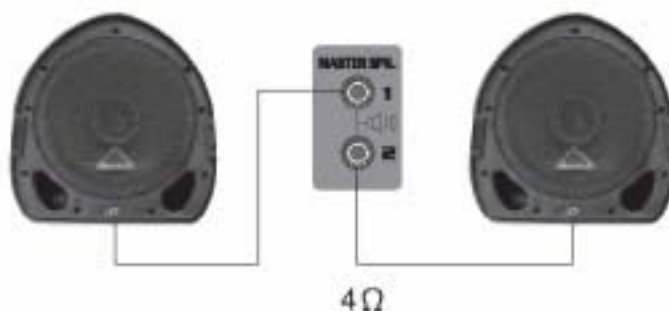
Connecting two speakers
