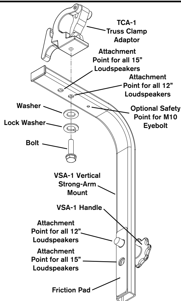
Figure 2: Assembling the TCA-1 to the VSA-1
