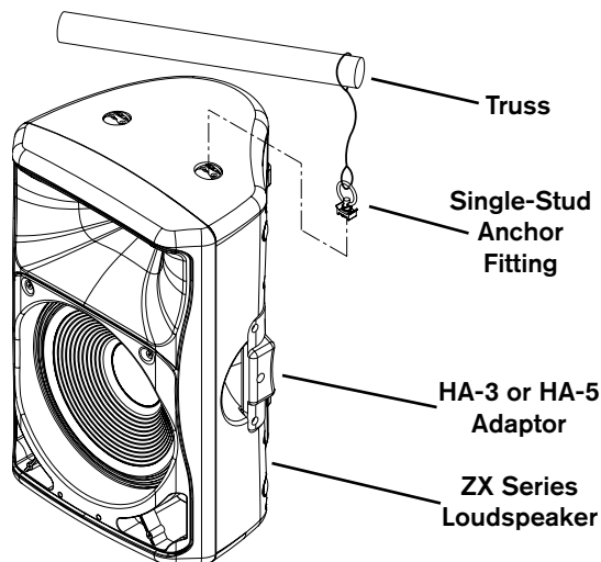
Figure 9: Attaching a Safety Point to a ZX Series Loudspeaker (VSA-1 Not Shown for Clarity)
