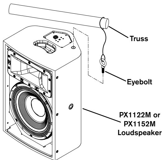
Figure 7: Attaching a Safety Point to a Phoenix Series Loudspeaker (VSA-1 Not Shown for Clarity)
