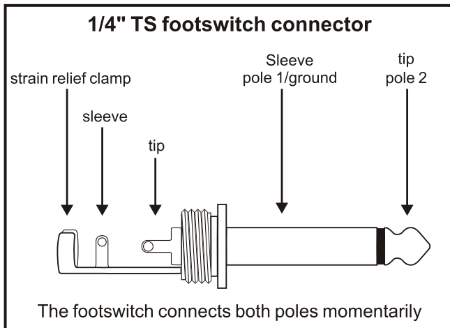
Foot switch connector
